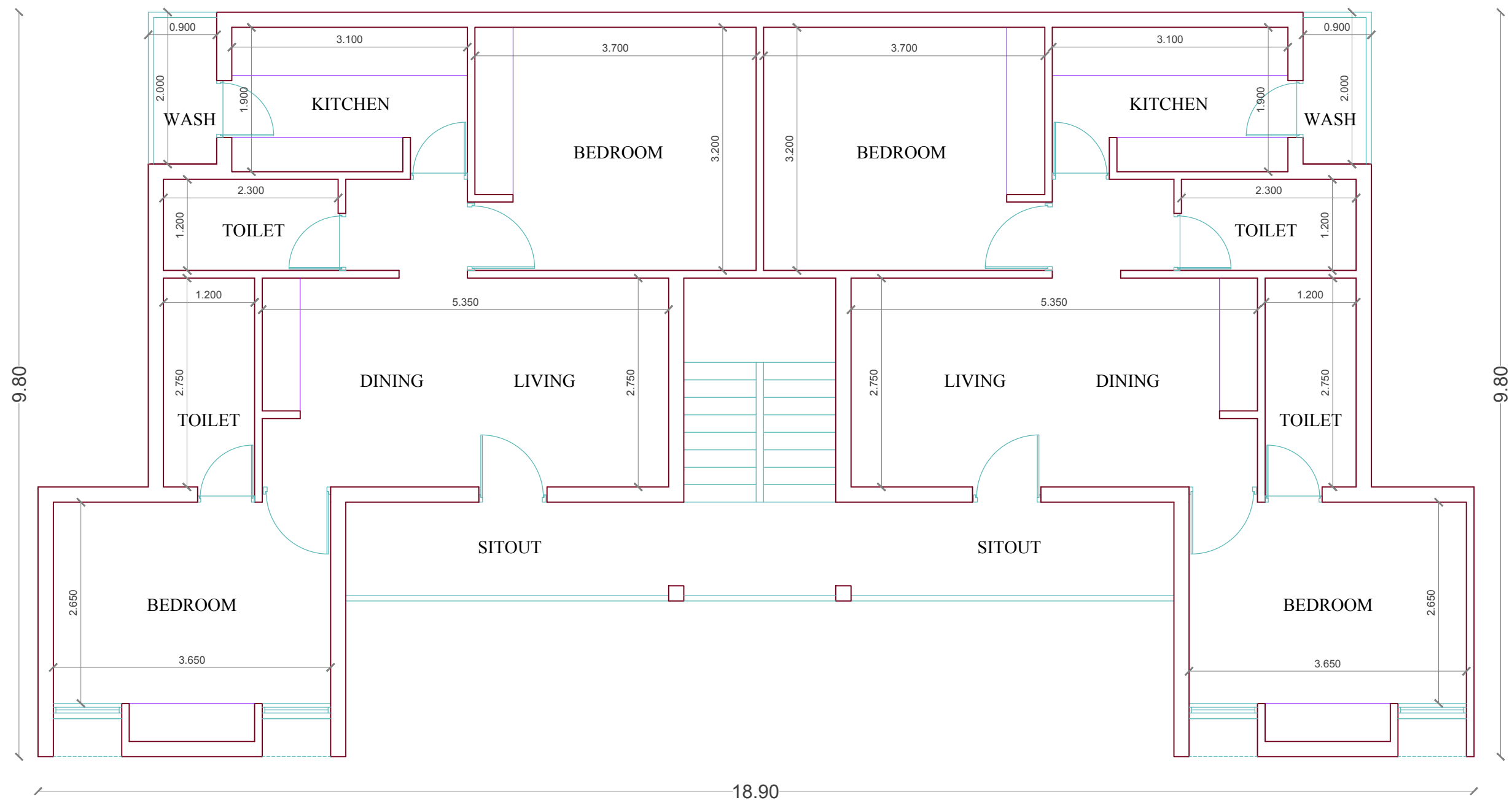
TYPICAL FLOOR
